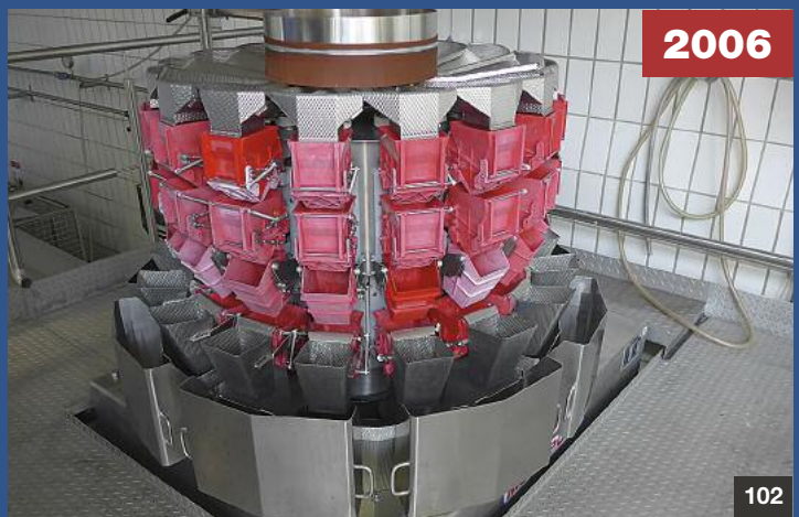
"MULTIPOND" MP 1601-FFC-S5R (4x4) (2006) Mehrkopf-Wägeautomat • multihead weigher
